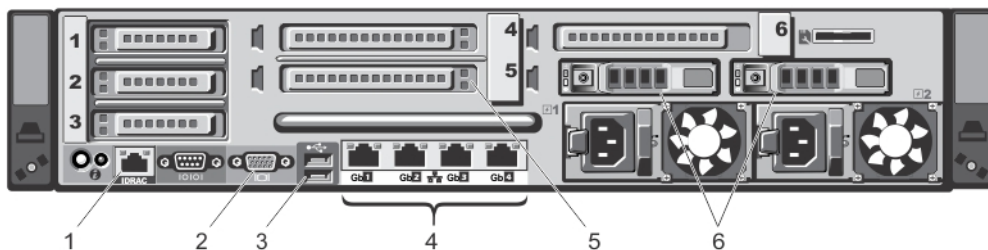
Figure 7. DR4100 System Rear Chassis Port Locations
