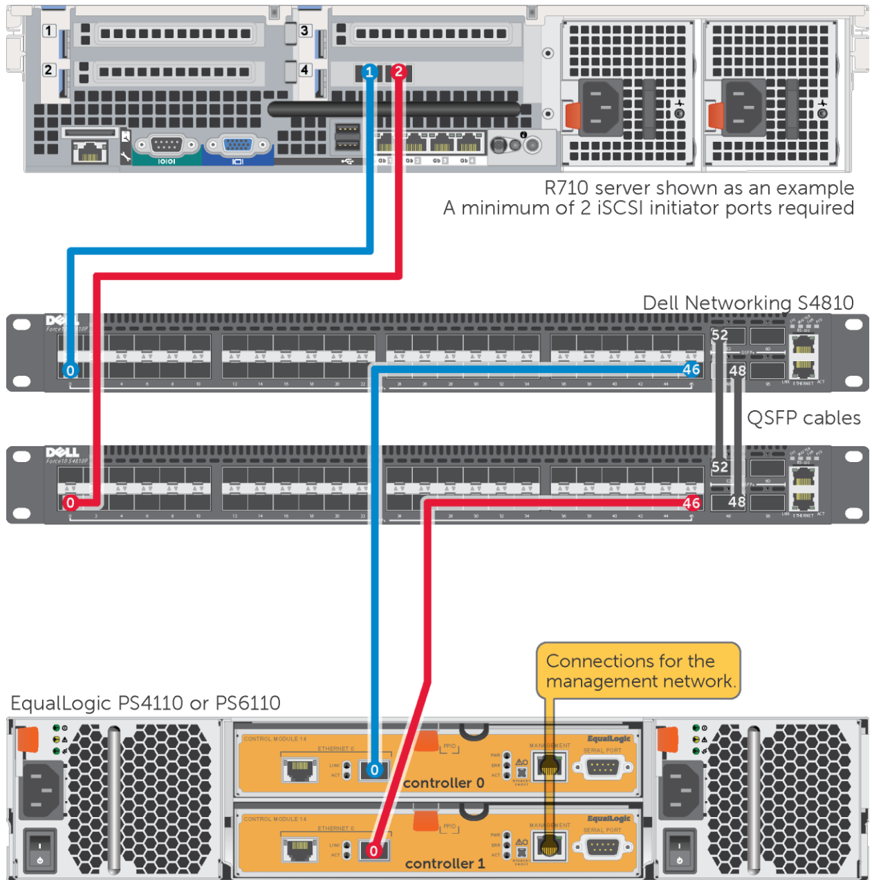
Figure 1 Dell Networking S4810 and EqualLogic PS4110 or PS6110 configuration (table on page 14)
