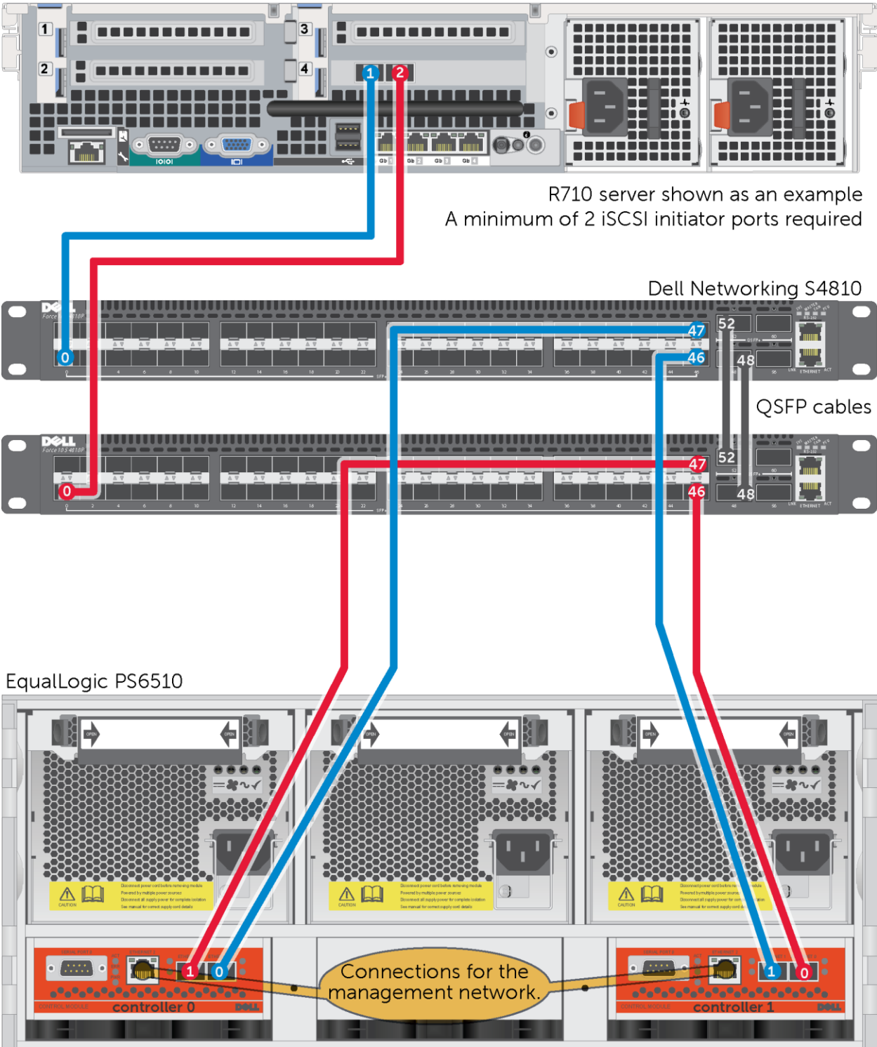
Figure 4 Dell Networking S4810 and EqualLogic PS6510 configuration (table on page 14)
