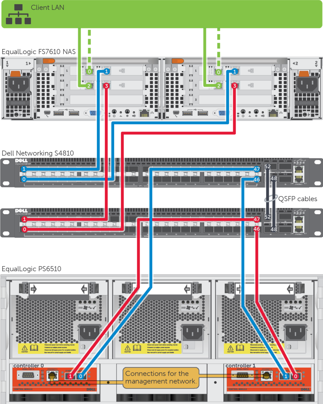
Figure 7 Dell Networking S4810 connections with the EqualLogic FS7610 and PS6510 (table on page 15)
