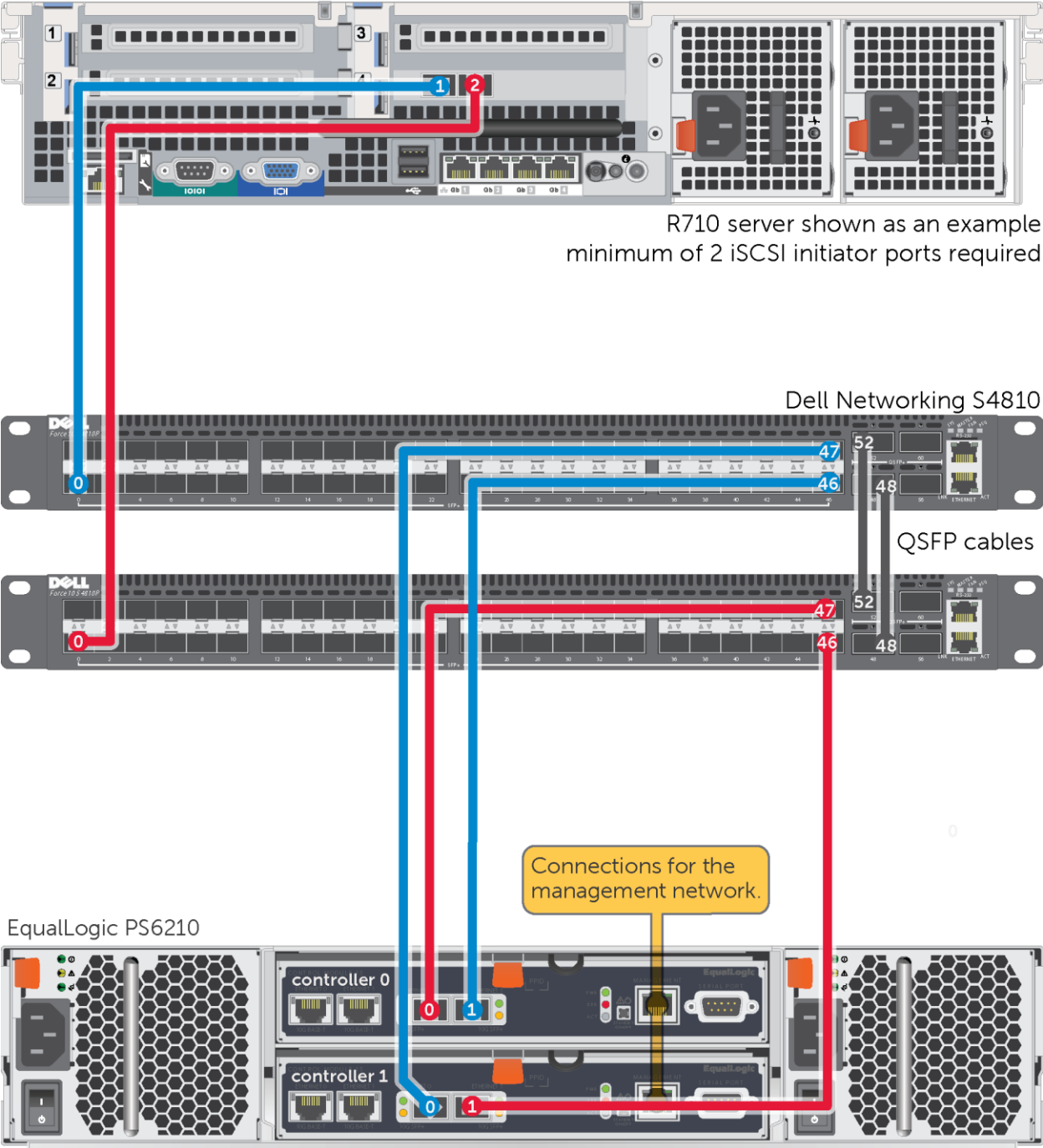
Figure 3 Dell Networking S4810 and EqualLogic PS6210 configuration (table on page 14)
