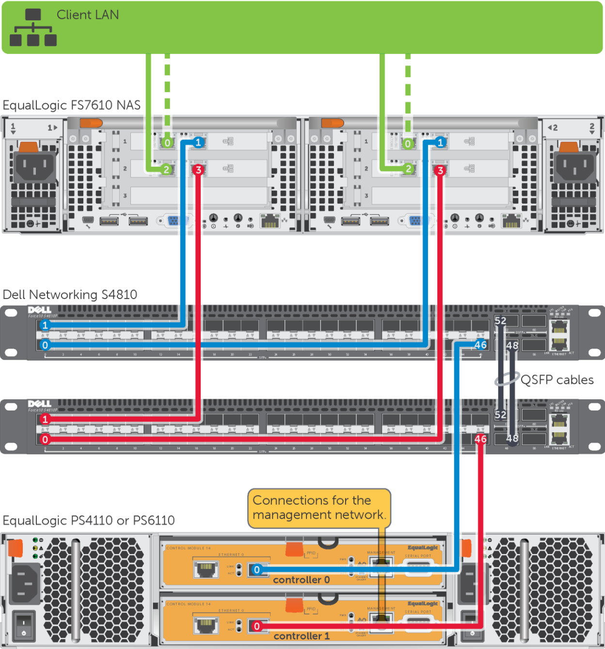
Figure 5 Dell Networking S4810 connections with the EqualLogic FS7610 and PS4110 or PS6110 (table on page 14)
