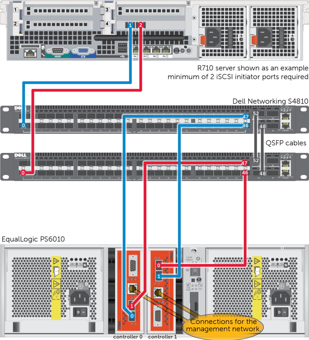
Figure 2 Dell Networking S4810 and EqualLogic PS6010 configuration (table on page 14)
