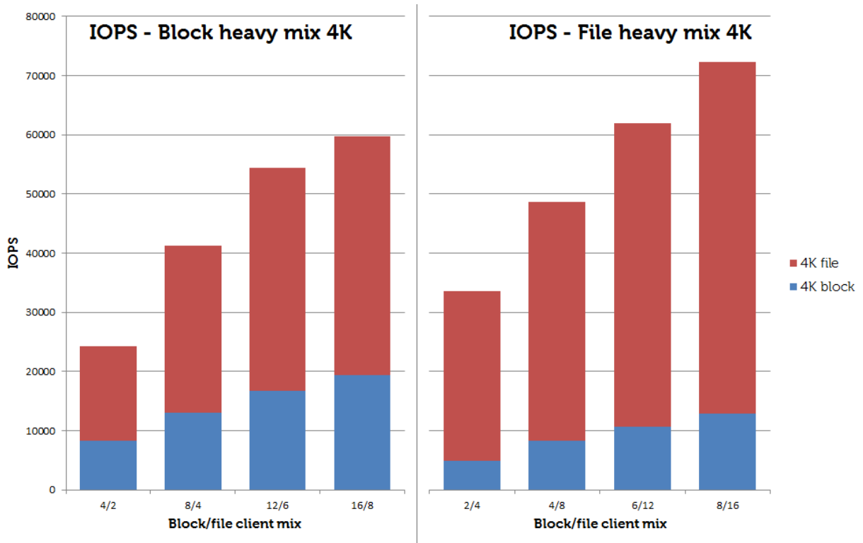
Figure 4 4K IOPS performance with FS7600 in separate pools
