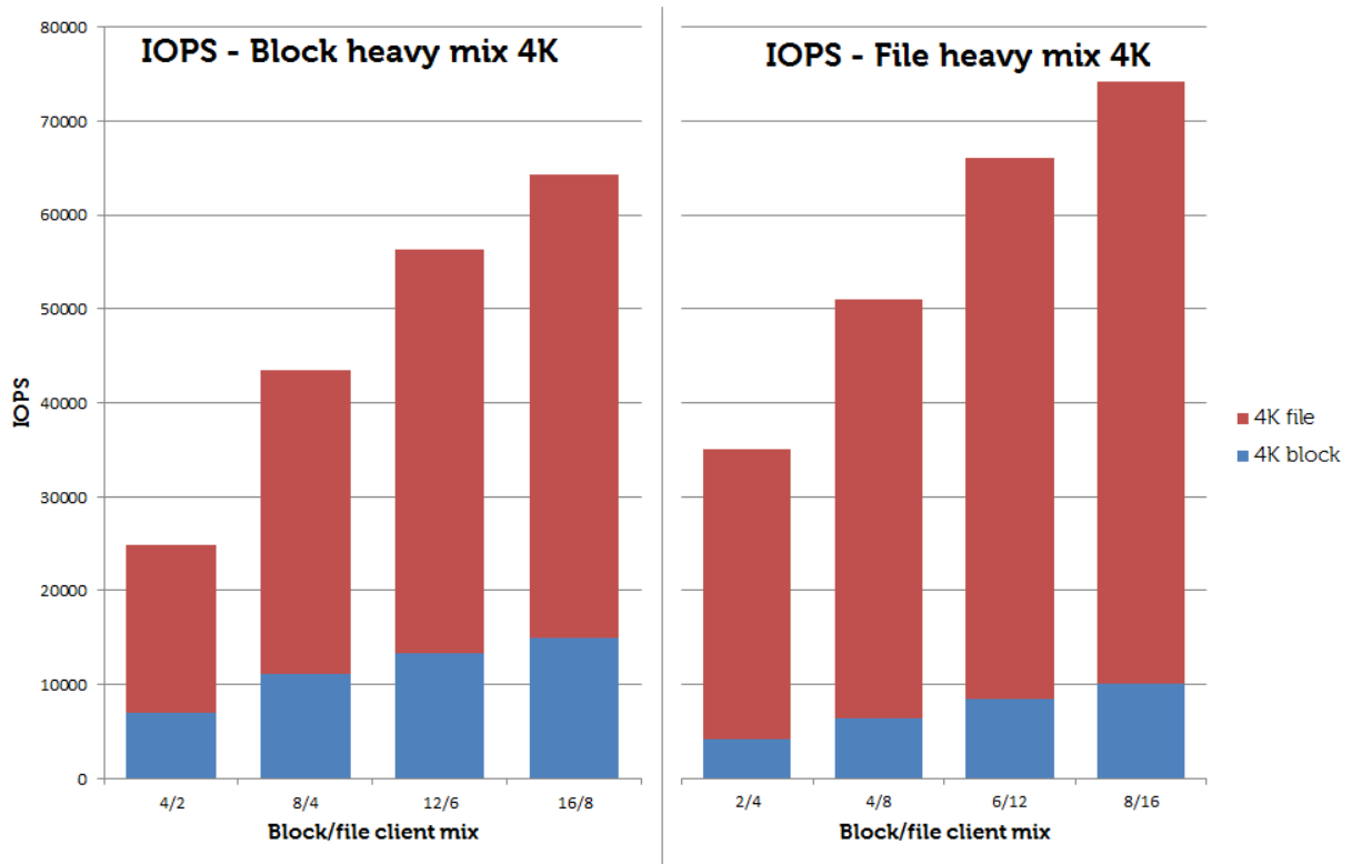
Figure 3 4K IOPS performance with FS7600 in shared pool
