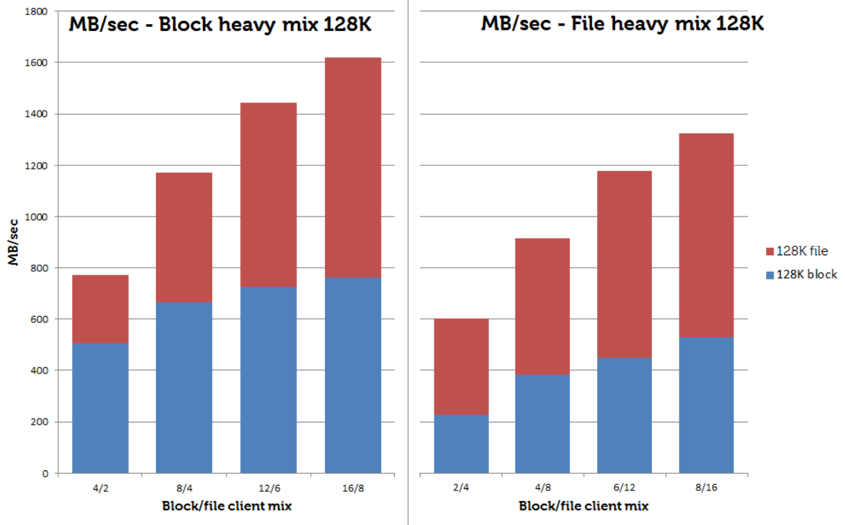
Figure 5 Throughput (MB/sec) with 128K I/O request in shared pool
