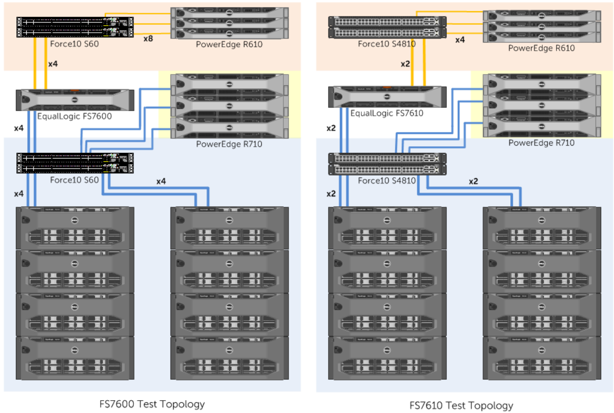
Figure 9 Test topology diagrams
