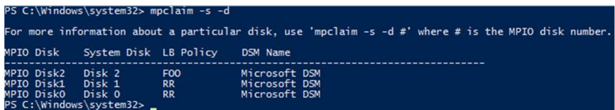
Figure 5 Listing MPIO volumes
