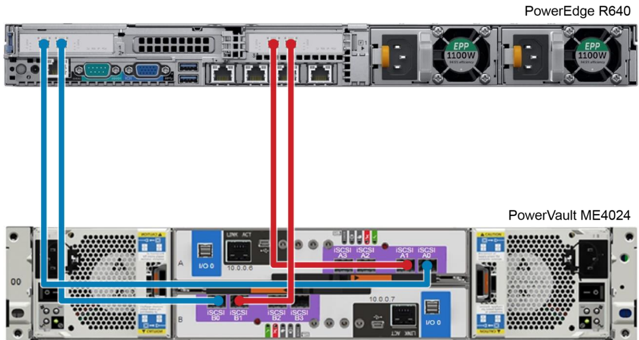
Figure 2 Single-server configuration cabling diagram
