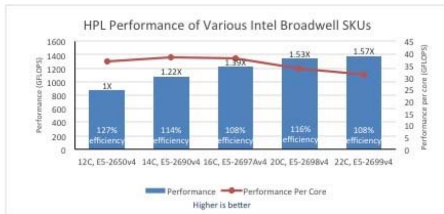
Figure1: HPL performance characterization
