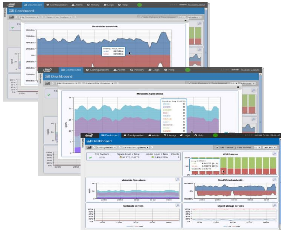
Figure 8: Intel Manager for Lustre (IML) interface
