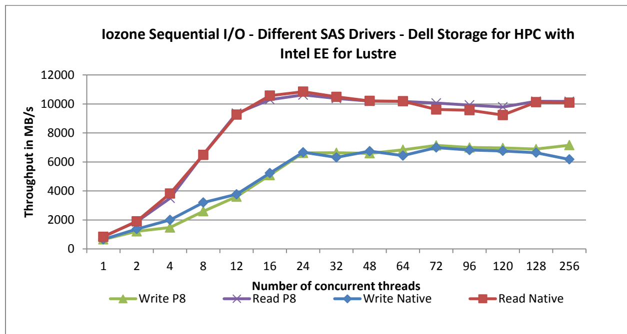
Figure 12: SAS drivers
