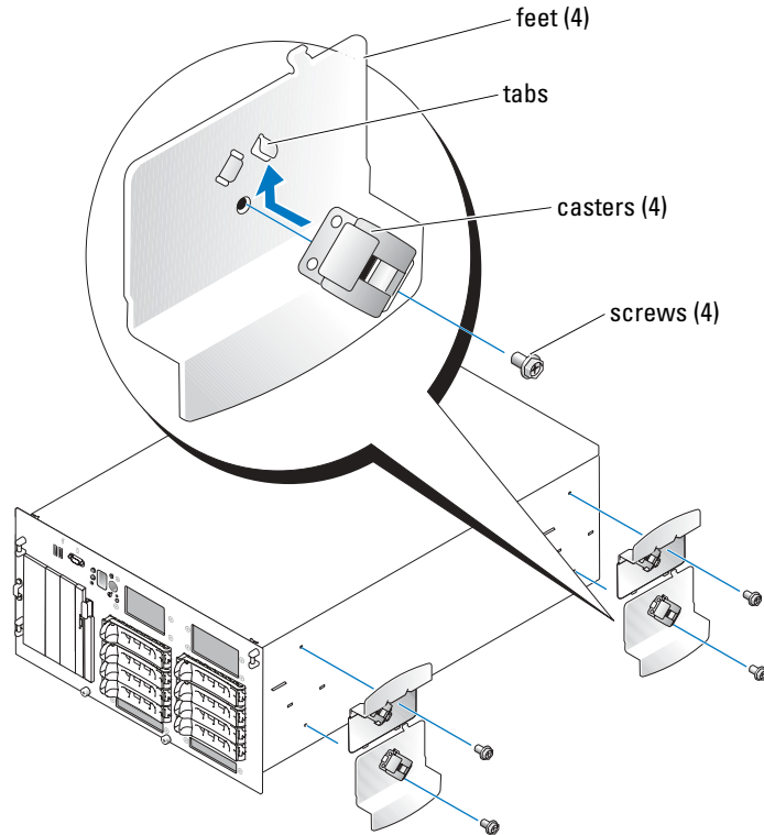
Figure 1. Attaching Casters to Your System
