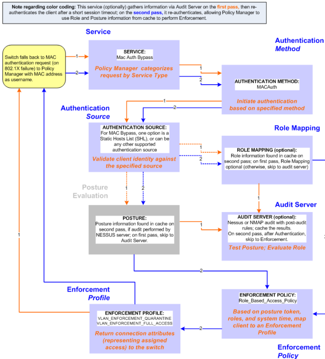
Figure 3: Flow-of-Control of MAC Authentication for Network Devices
