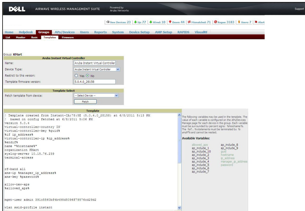
Figure 96 Template-based Configuration
