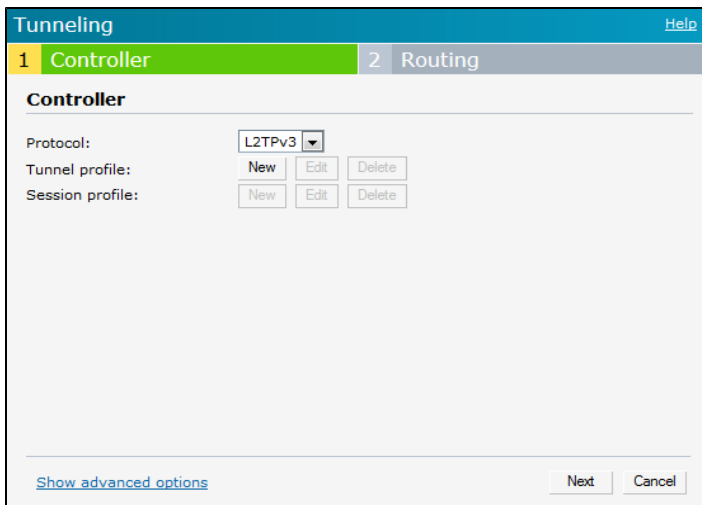
Figure 67 L3TPv3 Tunneling
