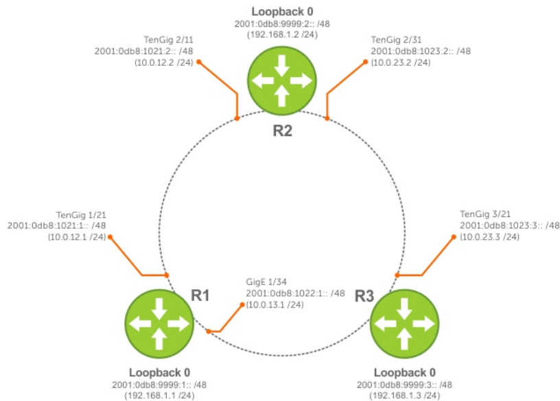
Figure 60. IPv6 IS-IS Sample Topology
