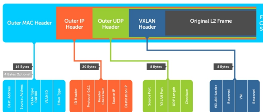
Figure 149. VXLAN Frame Format
