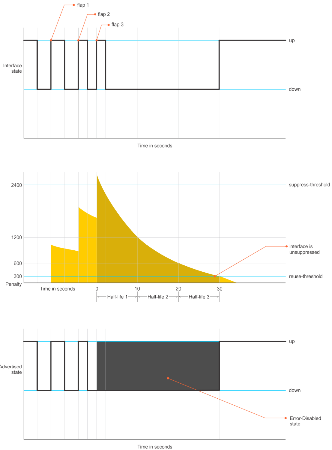
Figure 48. Interface State Change
