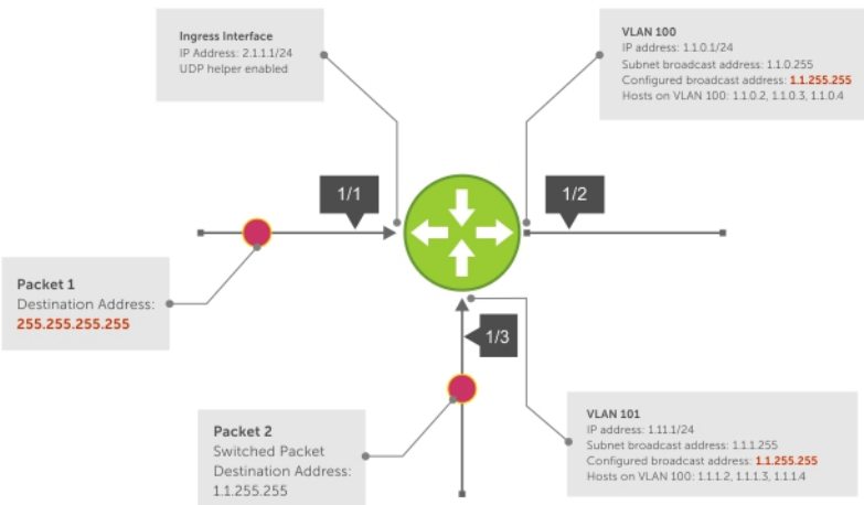
Figure 54. UDP Helper with Configured Broadcast Addresses
