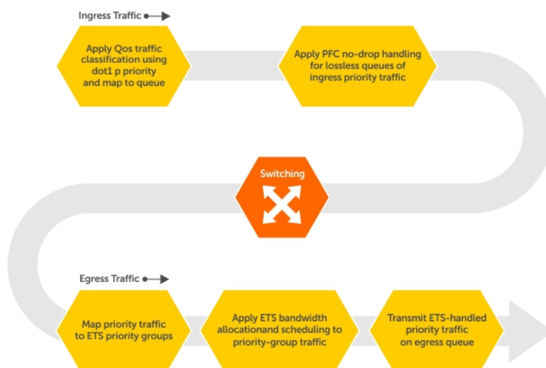
Figure 31. DCB PFC and ETS Traffic Handling
