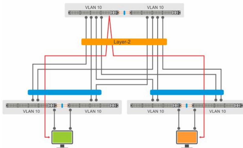
Figure 135. Layer-2 Traffic in VLT Domains
