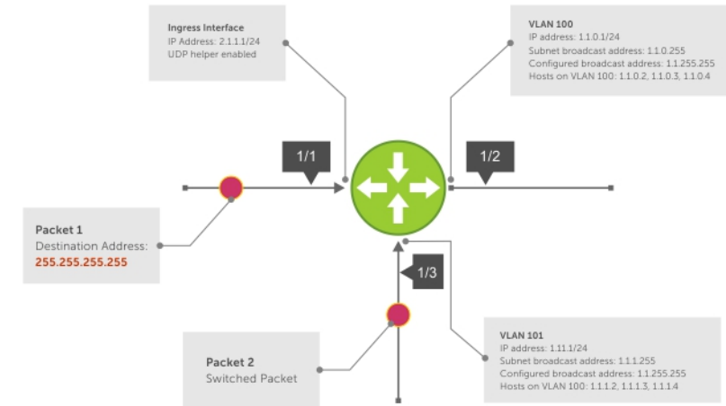
Figure 52. UDP Helper with Broadcast-All Addresses
