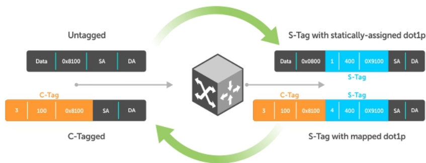
Figure 119. Statically and Dynamically Assigned dot1p for VLAN Stacking
