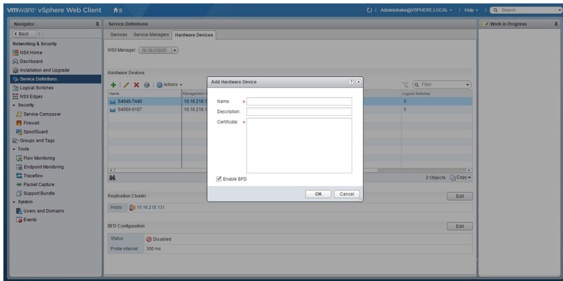
Figure 150. Create VXLAN Gateway
