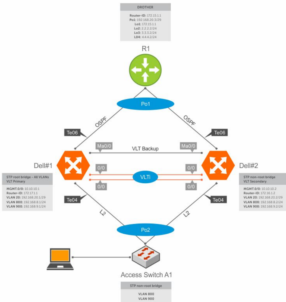
Figure 141. Peer Routing Configuration Example
