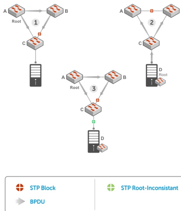
Figure 125. STP Root Guard Prevents Bridging Loops
