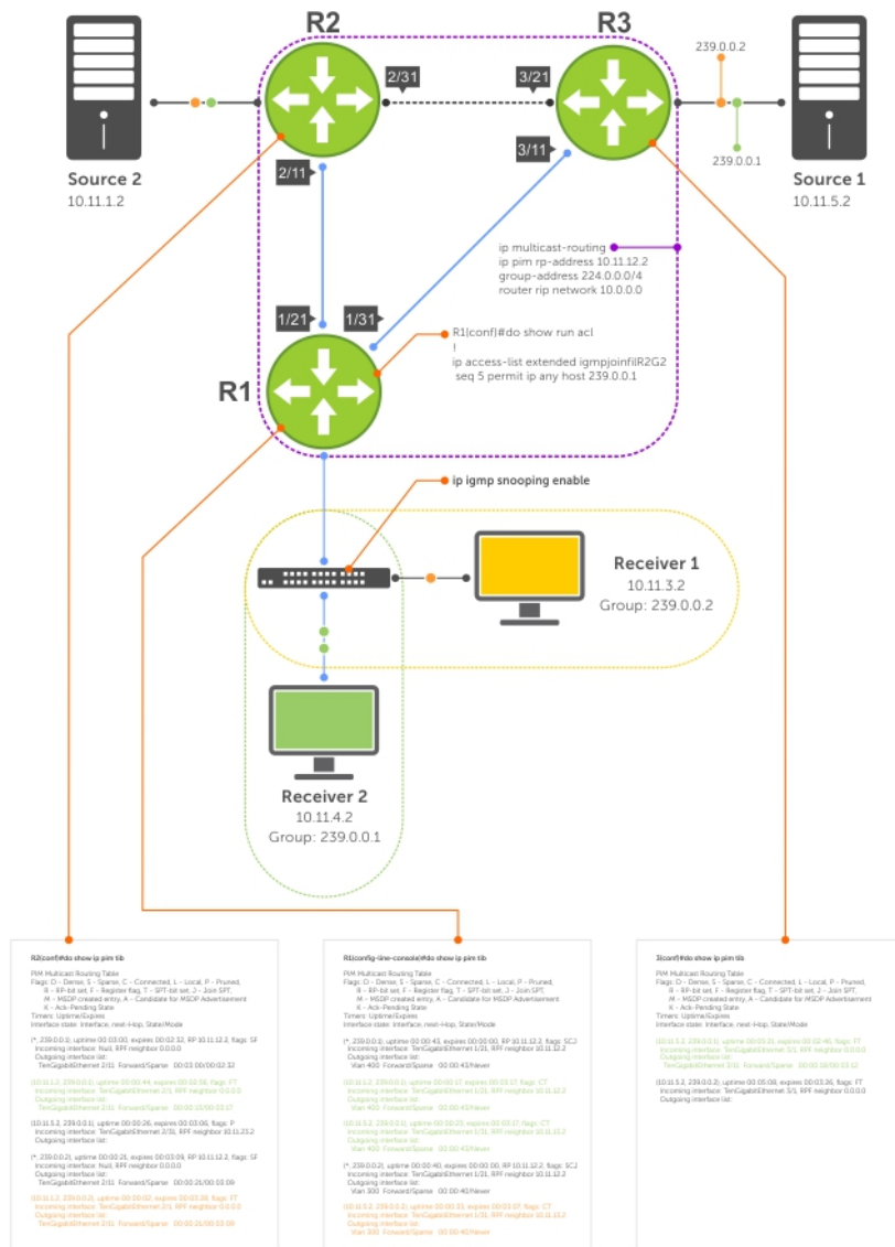
Figure 95. Preventing a Source from Transmitting to a Group
