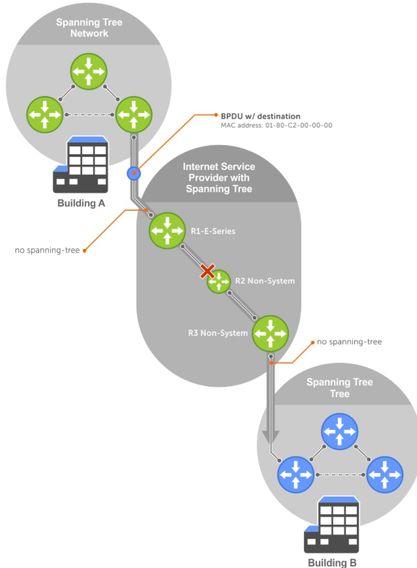
Figure 120. VLAN Stacking without L2PT
