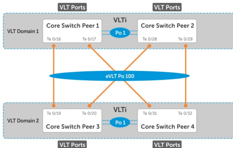
Figure 142. eVLT Configuration Example
