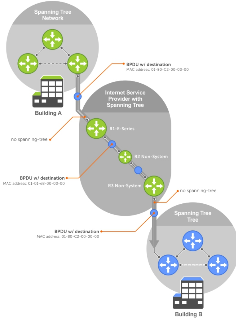
Figure 121. VLAN Stacking with L2PT
