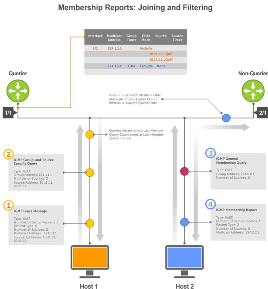
Figure 47. Membership Queries: Leaving and Staying
