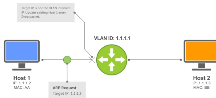
Figure 49. ARP Learning via ARP Request
