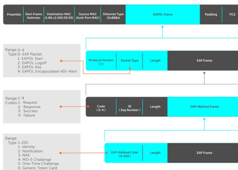
Figure 4. EAP Frames Encapsulated in Ethernet and RADIUS
