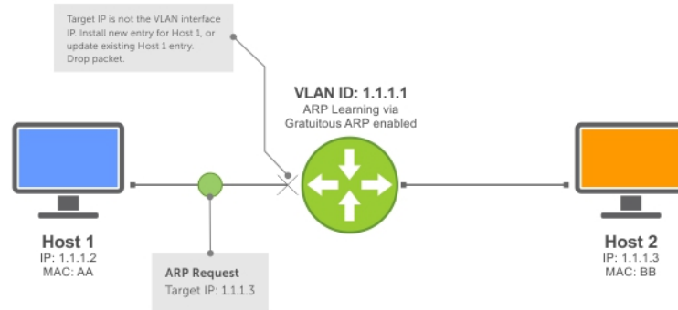
Figure 50. ARP Learning via ARP Request with ARP Learning via Gratuitous ARP Enabled
