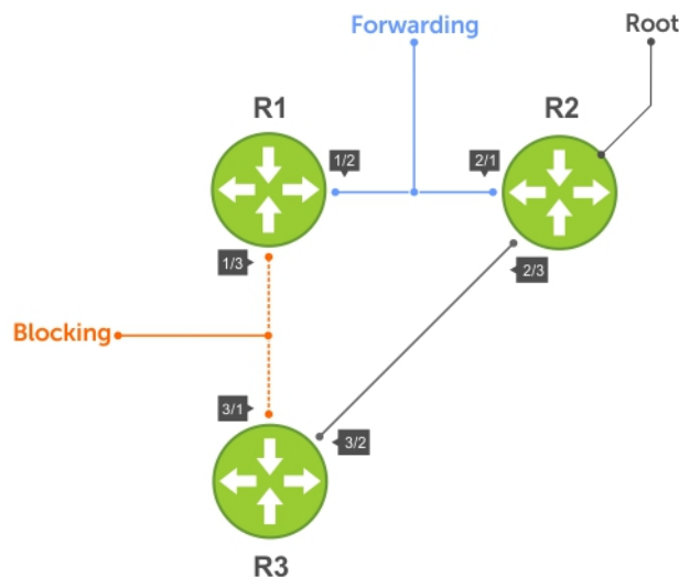
Figure 93. MSTP with Three VLANs Mapped to Two Spanning Tree Instances
