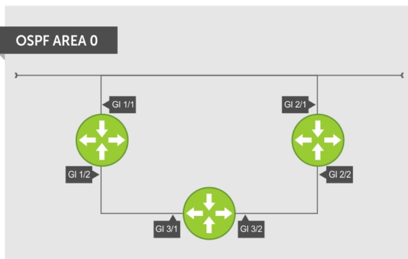
Figure 100. Basic Topology and CLI Commands for OSPFv2
