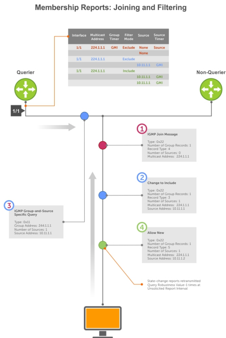
Figure 46. Membership Reports: Joining and Filtering
