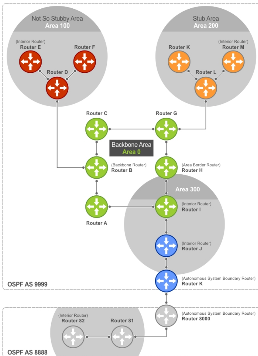
Figure 98. OSPF Routing Examples
