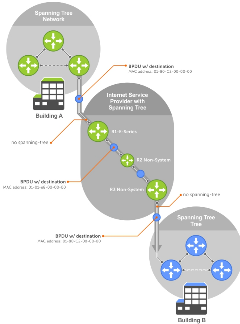
Figure 120. VLAN Stacking with L2PT
