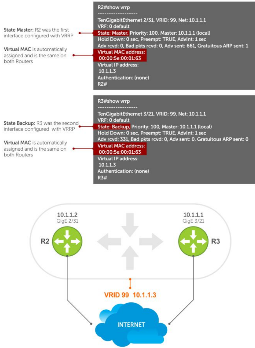
Figure 172. VRRP for IPv4 Topology
