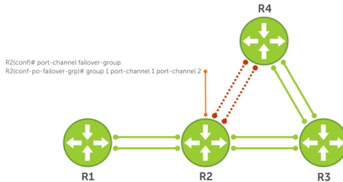
Figure 65. Configuring Shared LAG State Tracking
