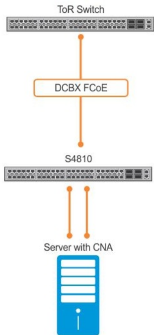
Figure 40. Configuration Example: FIP Snooping on a Switch
