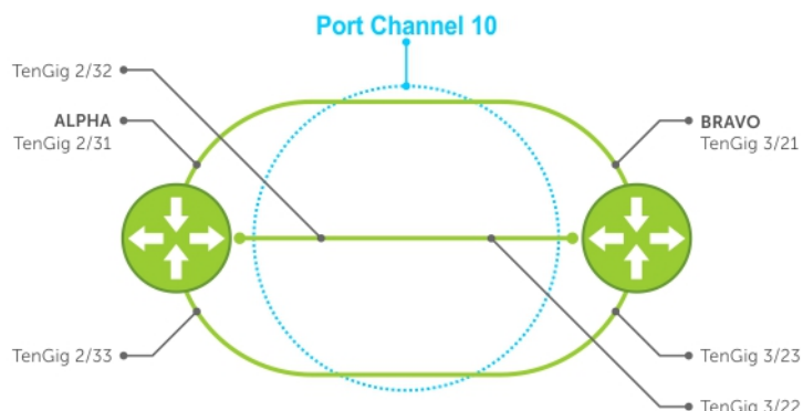
Figure 66. LACP Basic Configuration Example
