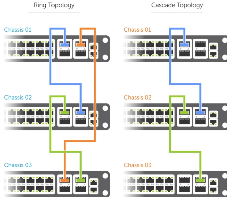
Figure 125. Supported Stacking Topologies
