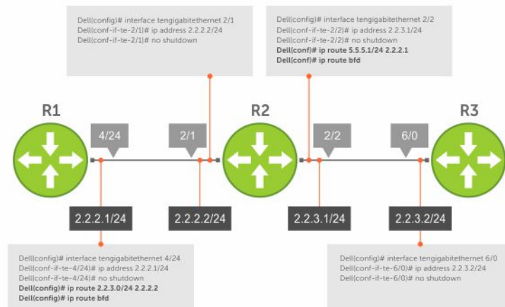
Figure 17. Establishing Sessions for Static Routes
