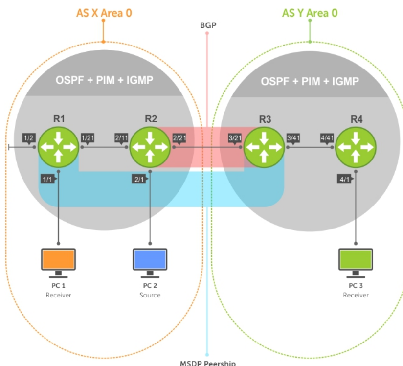
Figure 85. Multicast Source Discovery Protocol (MSDP)
