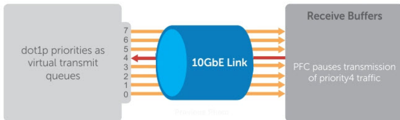
Figure 30. Illustration of Traffic Congestion
