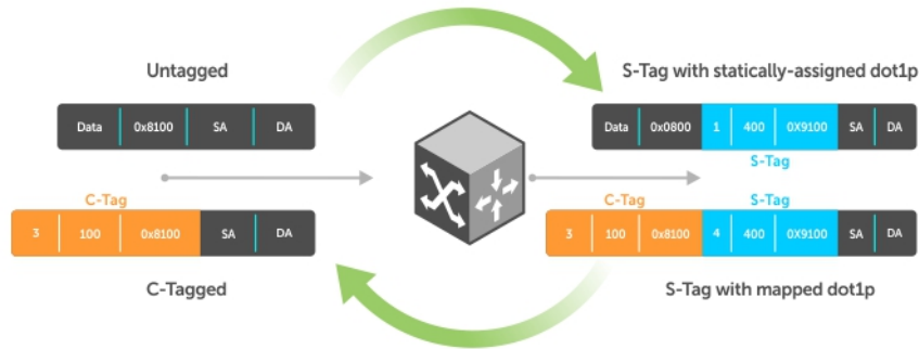
Figure 122. Statically and Dynamically Assigned dot1p for VLAN Stacking
