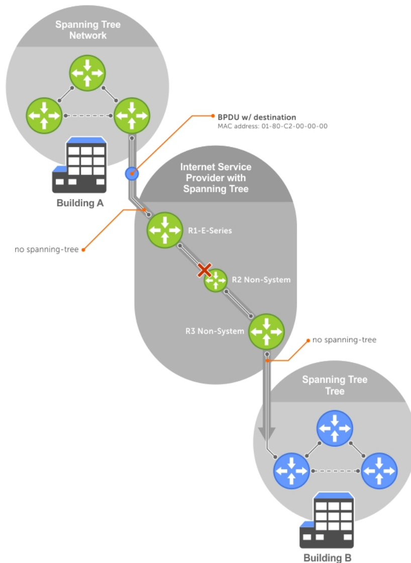
Figure 123. VLAN Stacking without L2PT
