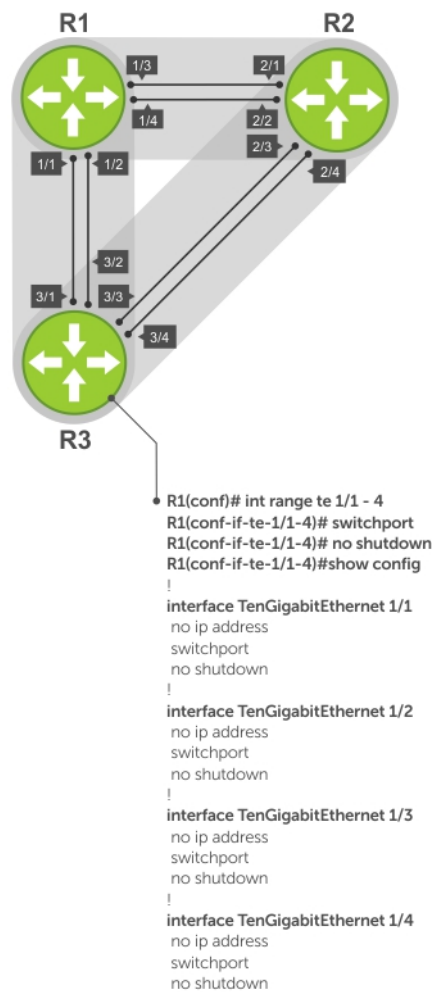
Figure 128. Example of Configuring Interfaces for Layer 2 Mode
