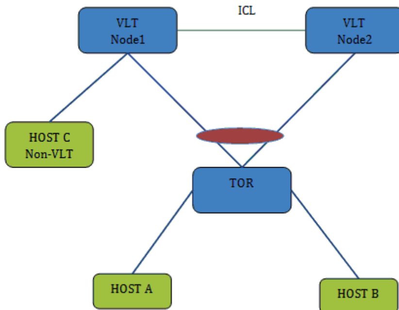
Figure 148. Sample Configuration of IPv6 Peer Routing in a VLT Domain
