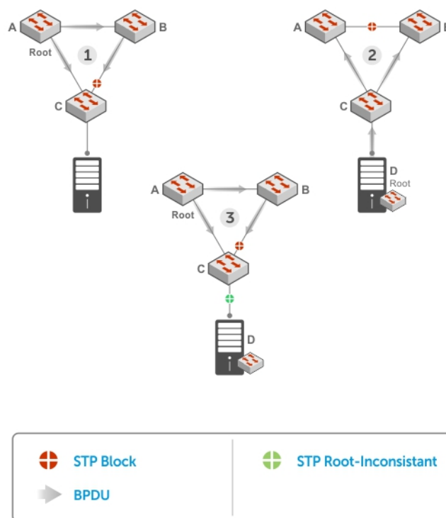
Figure 131. STP Root Guard Prevents Bridging Loops
