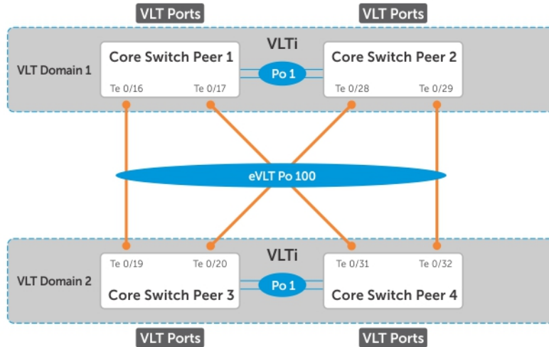
Figure 146. eVLT Configuration Example
