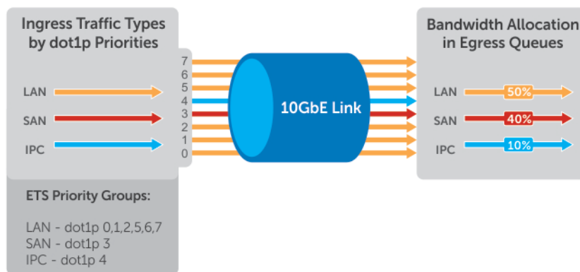
Figure 31. Enhanced Transmission Selection
