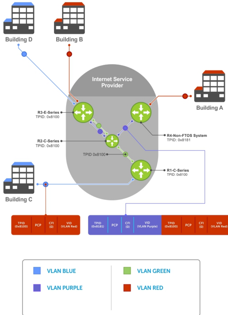
Figure 119. Single and Double-Tag TPID Match
