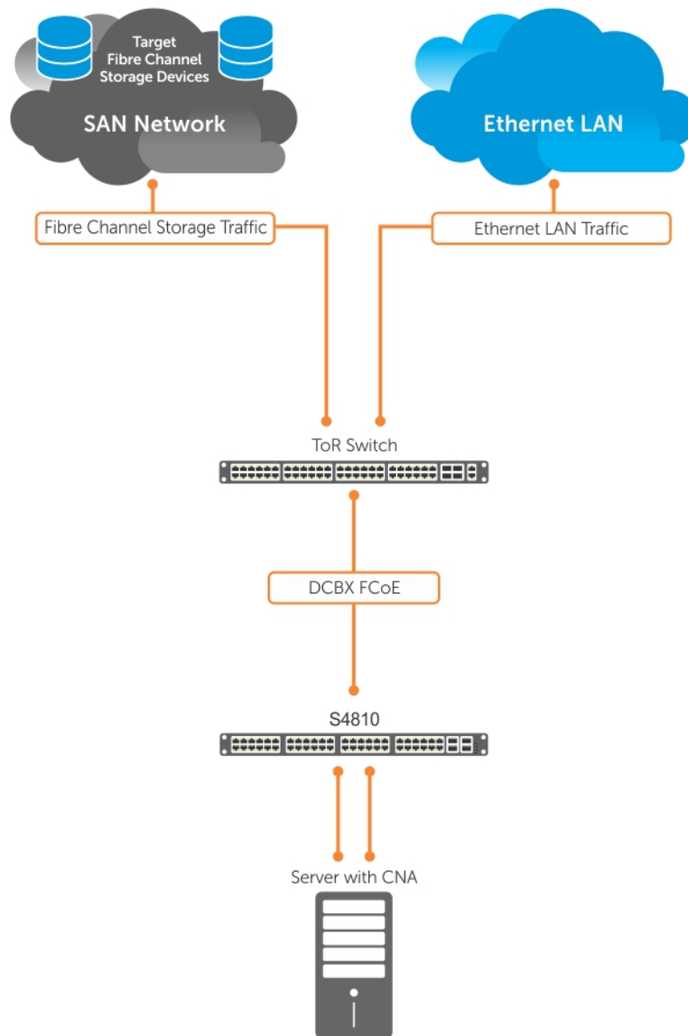
Figure 39. FIP Snooping on a Dell EMC Networking Switch
