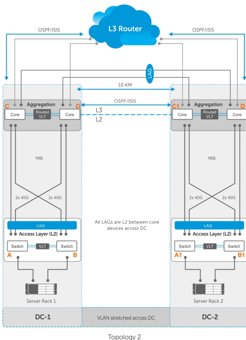
Figure 139. Sample Configuration for a VLT Proxy Gateway
