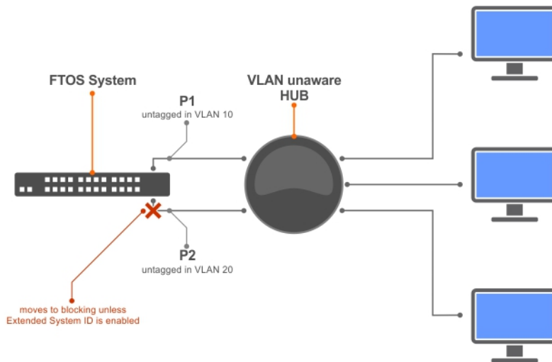
Figure 112. PVST+ with Extend System ID
