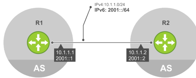
Figure 27. Configure IPv6 NH to advertise IPv6 prefix over IPv4 neighbor
