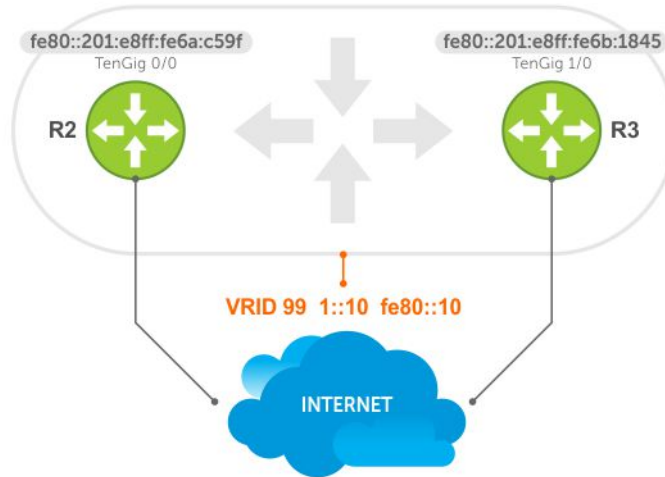
Figure 154. VRRP for an IPv6 Configuration
