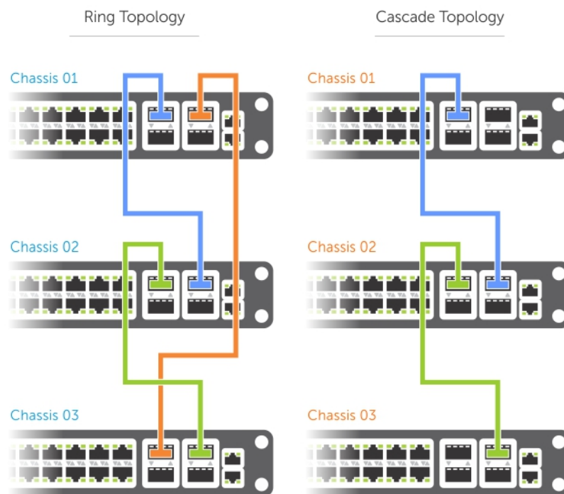
Figure 115. Supported Stacking Topologies
