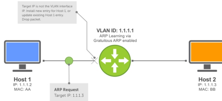
Figure 44. ARP Learning via ARP Request with ARP Learning via Gratuitous ARP Enabled
