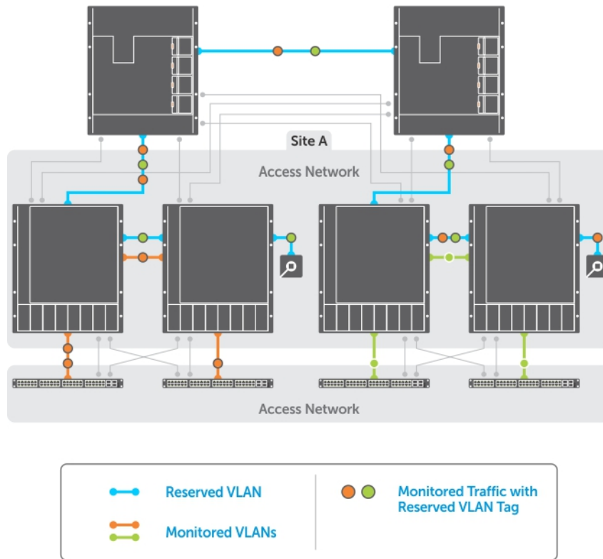
Figure 96. Remote Port Mirroring
