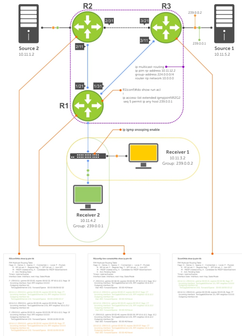
Figure 88. Preventing a Source from Transmitting to a Group
