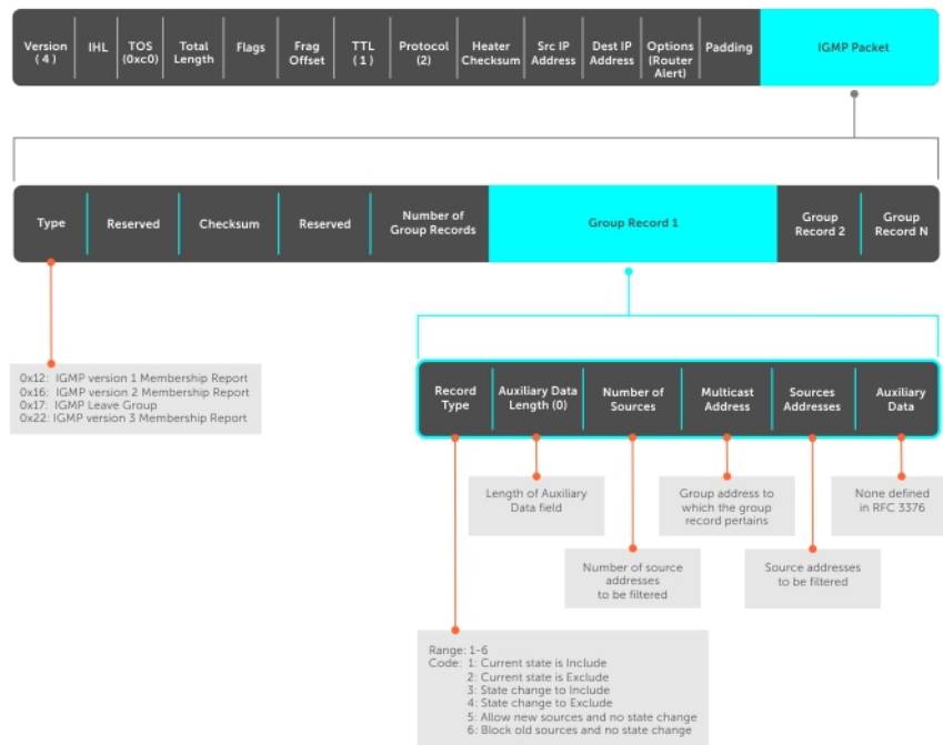
Figure 38. IGMP Version 3-Capable Multicast Routers Address Structure
