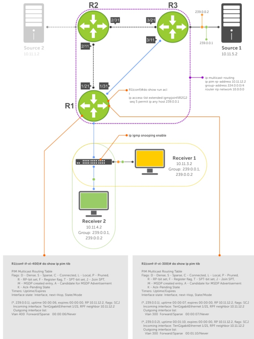
Figure 87. Preventing a Host from Joining a Group
