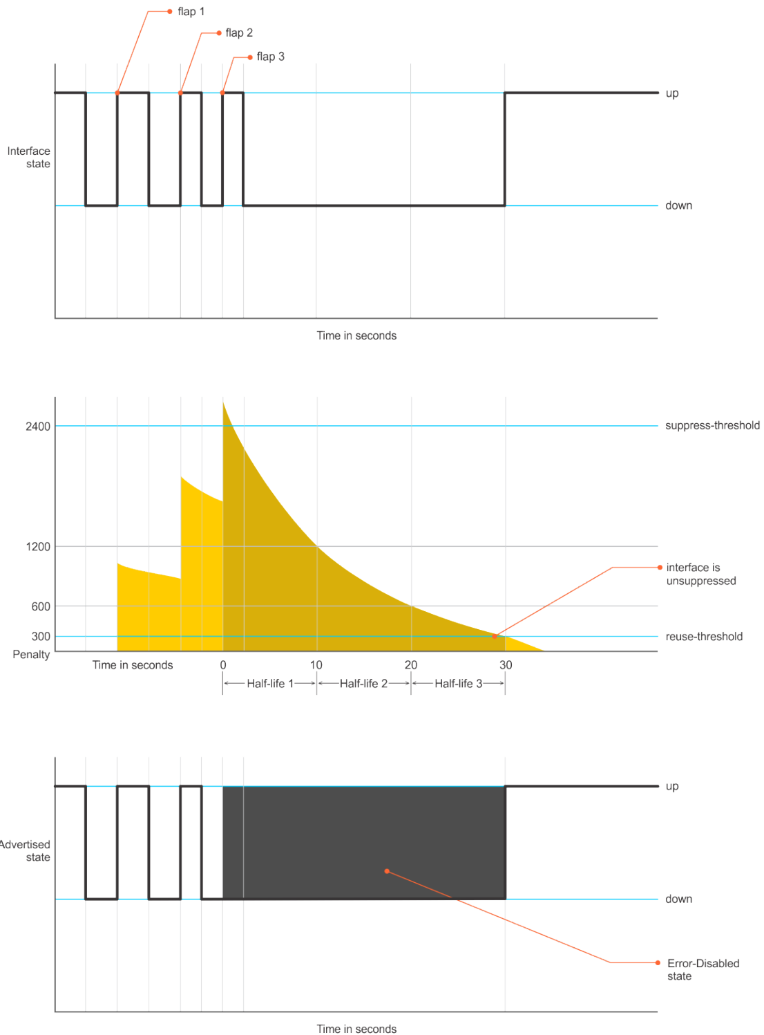
Figure 42. Interface State Change
