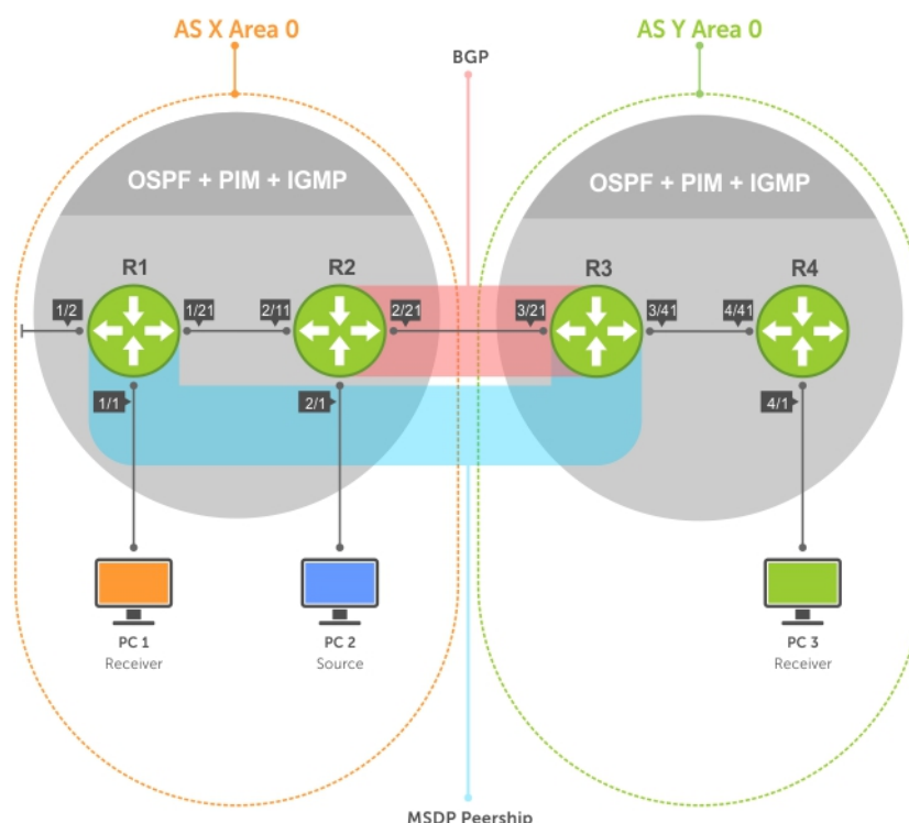
Figure 75. Multicast Source Discovery Protocol (MSDP)
