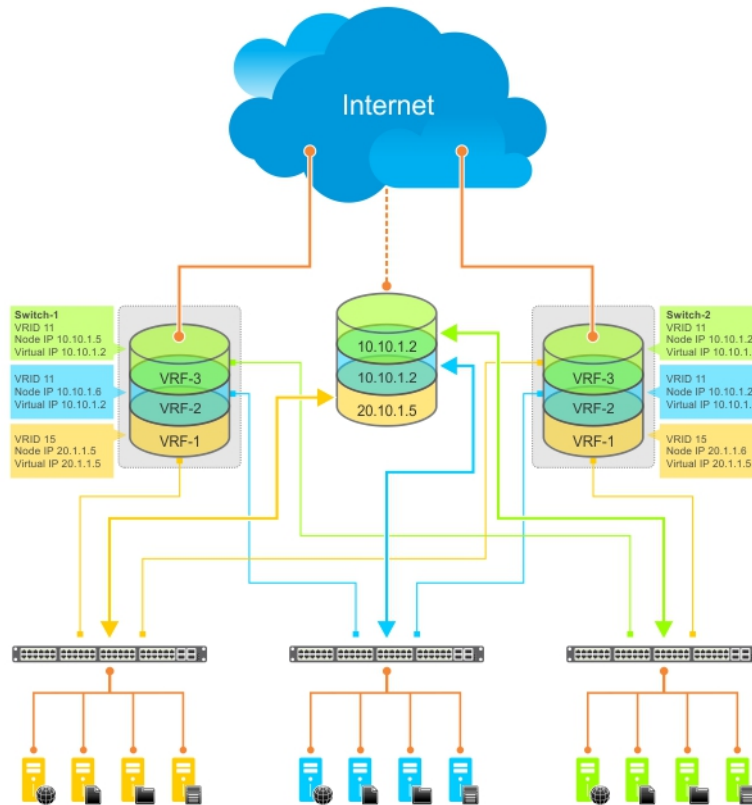
Figure 149. VRRP in a VRF: Non-VLAN Example
