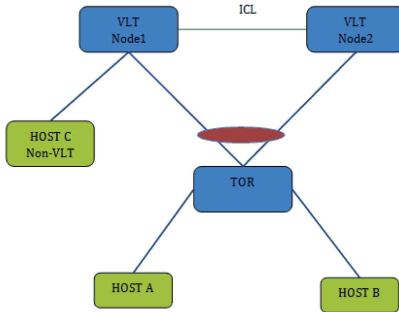
Figure 139. Sample Configuration of IPv6 Peer Routing in a VLT Domain
