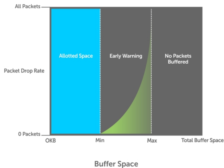
Figure 105. Packet Drop Rate for WRED
