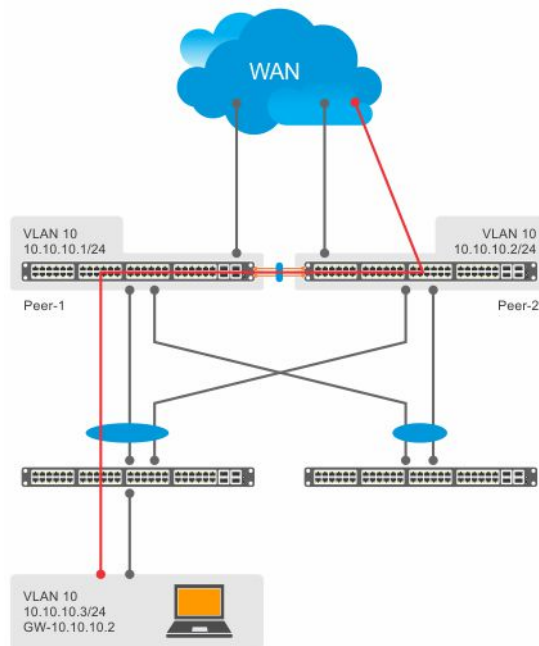
Figure 134. Packets without peer routing enabled
