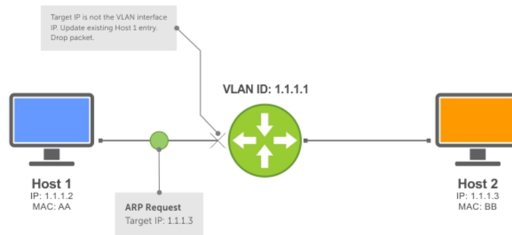
Figure 43. ARP Learning via ARP Request
