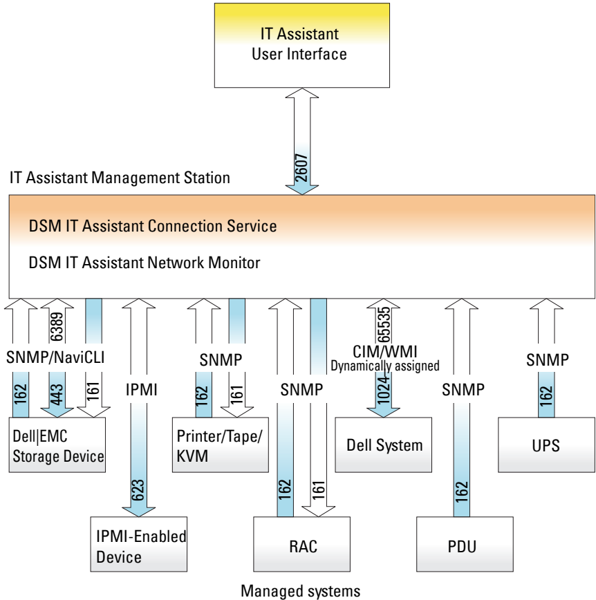
Figure 1-1. IT Assistant User Interface, Services System, and Managed System
