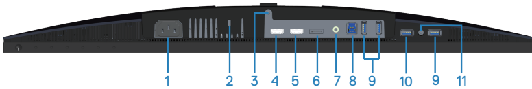
Bottom view without monitor stand (S2719DGF)
