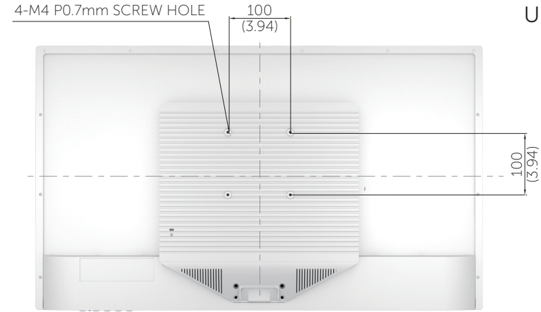
Back view of Monitor without stand
