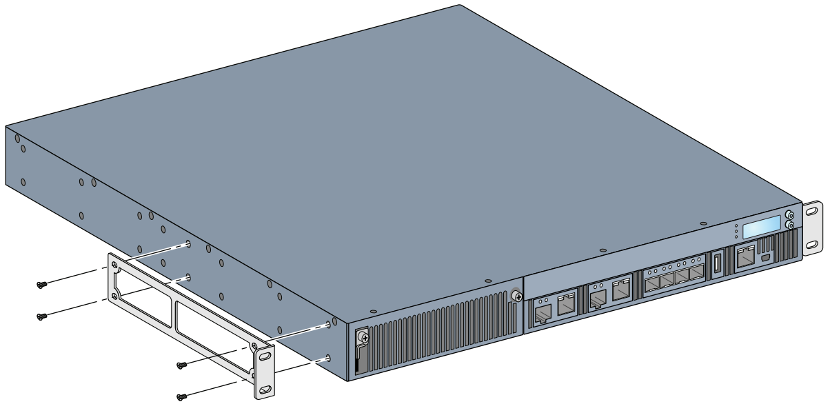
Figure 10 Rack Mount Brackets
