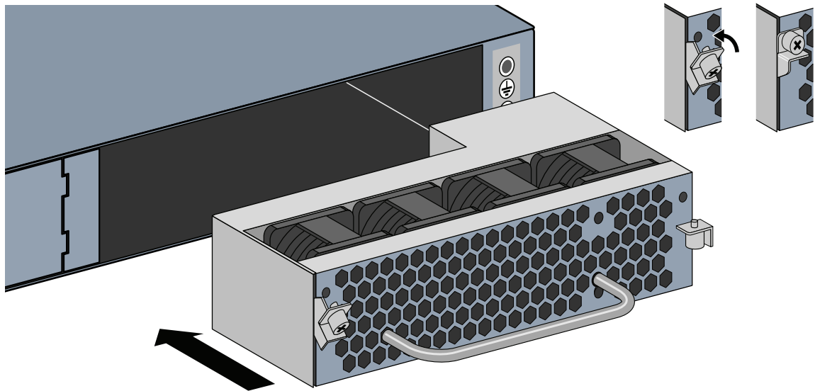
Figure 12 Installing a Fan Tray
