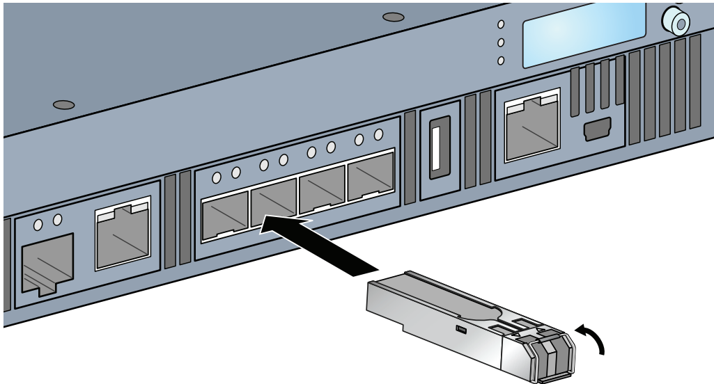
Figure 14 Installing an SFP
