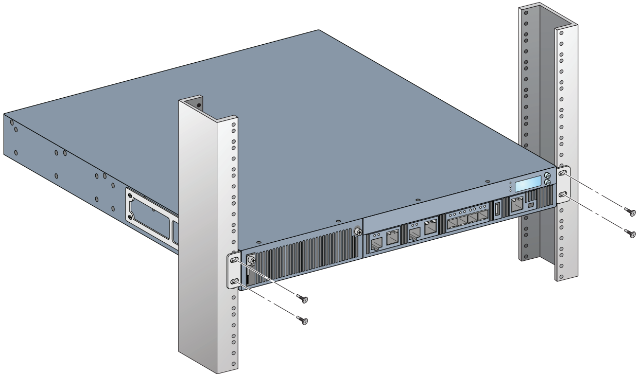
Figure 11 Rack Mount Installation
