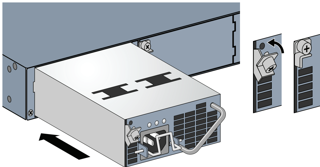
Figure 13 Installing a Power Supply
