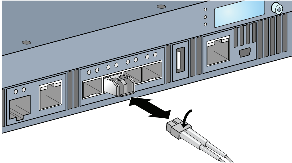
Figure 15 Connecting an LC Fiber Optic Cable
