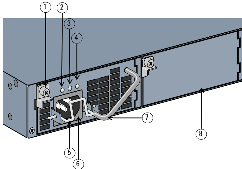
Figure 9 Power Supply (AC Power Supply Shown)
